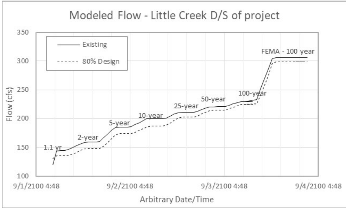
Figure 15. Modeled quasi-steady state hydrographs for existing and proposed conditions downstream of the Project site on Little Creek.
