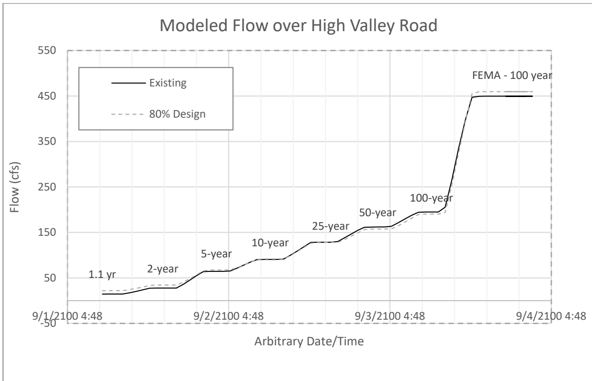
Figure 16. Modeled quasi-steady state hydrographs for existing and proposed conditions flowing over High Valley Road.
