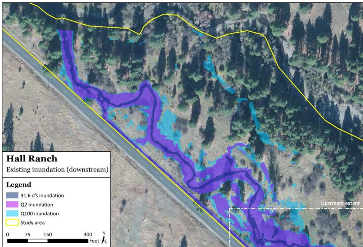
Figure 5. Modeled Inundation under Existing Conditions for the upstream and downstream portions of the side channel complex on the Hall Ranch property.
