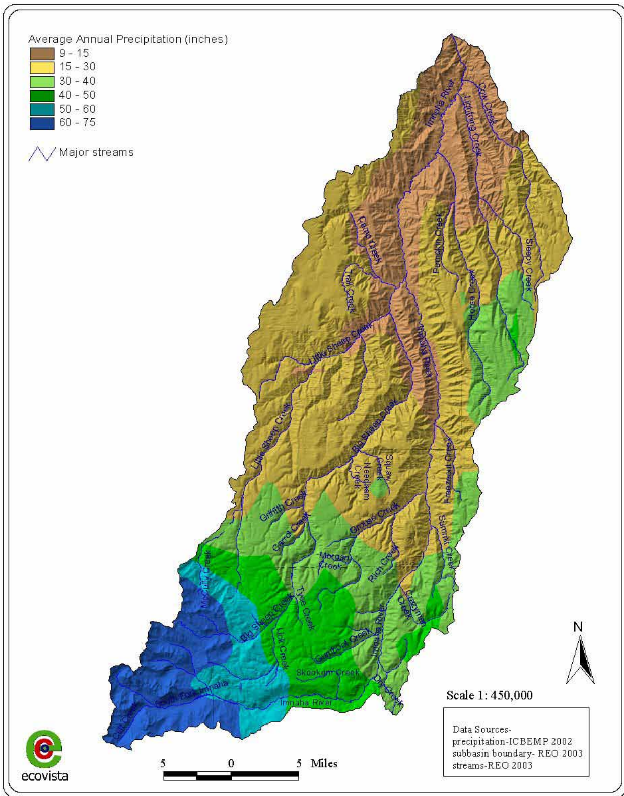
Figure 7. Precipitation patterns in the Imnaha subbasin.
